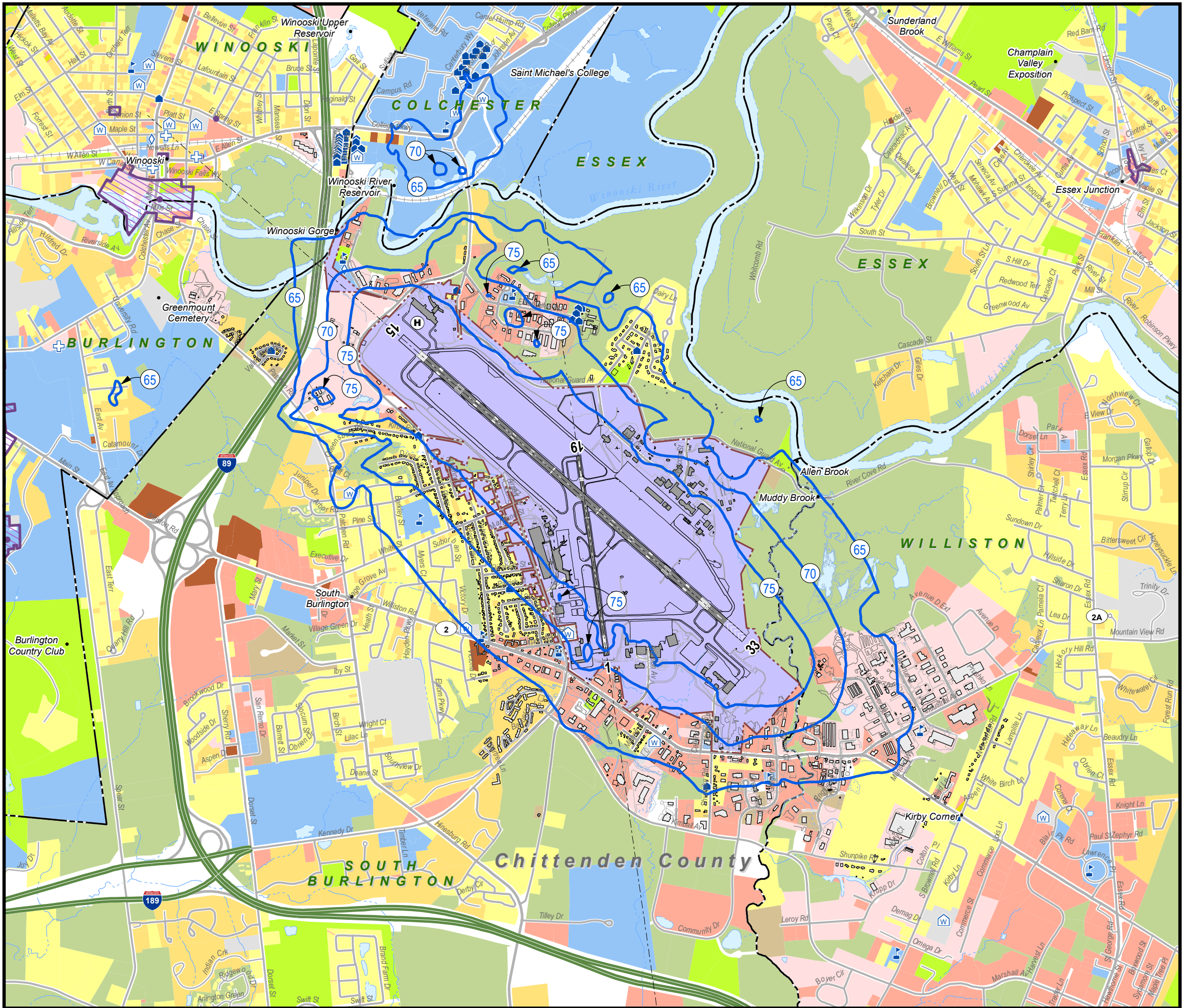
Figure 13 2020 Forecast Conditions Noise Exposure Map
